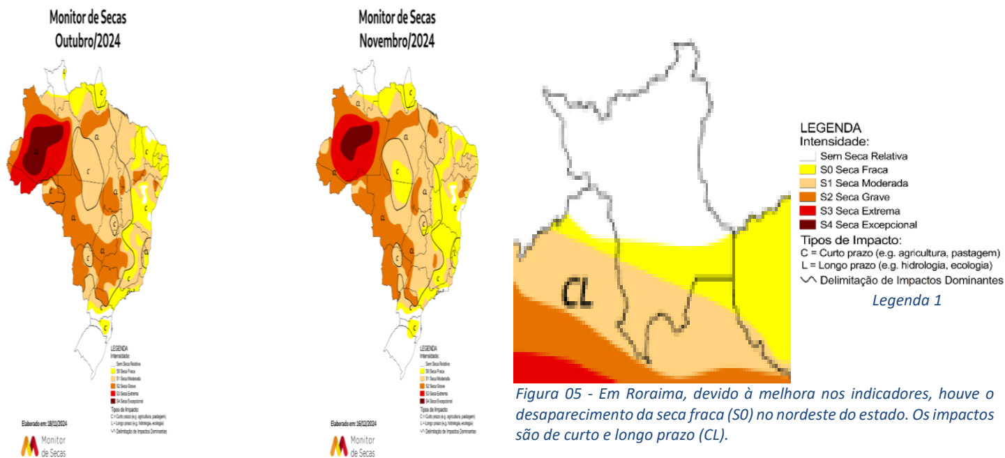
Figura 04 - Monitor de Secas: (a) out/2024, (b) nov/2024.
